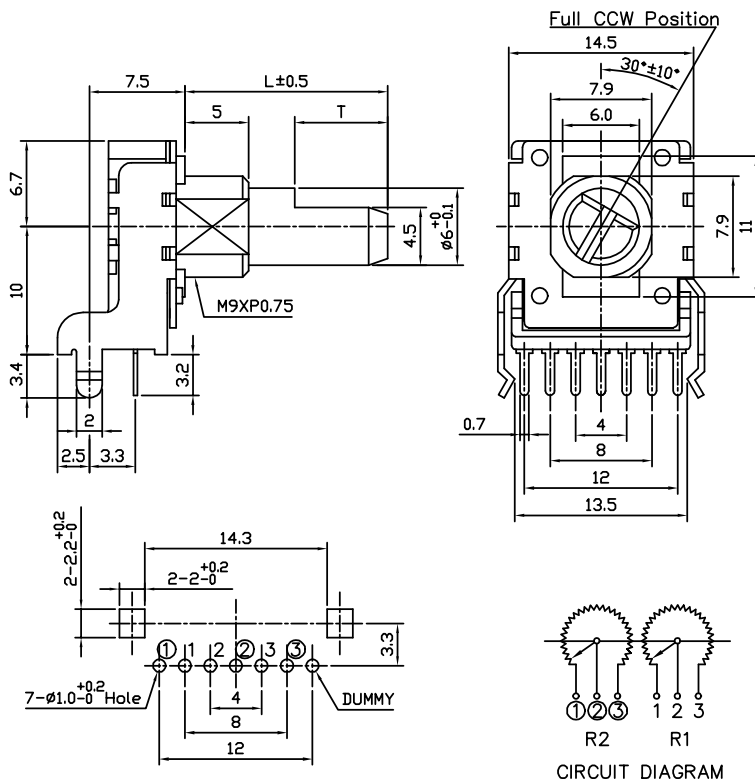
Model P140KV1 (Side Adjust, with Bushing)
