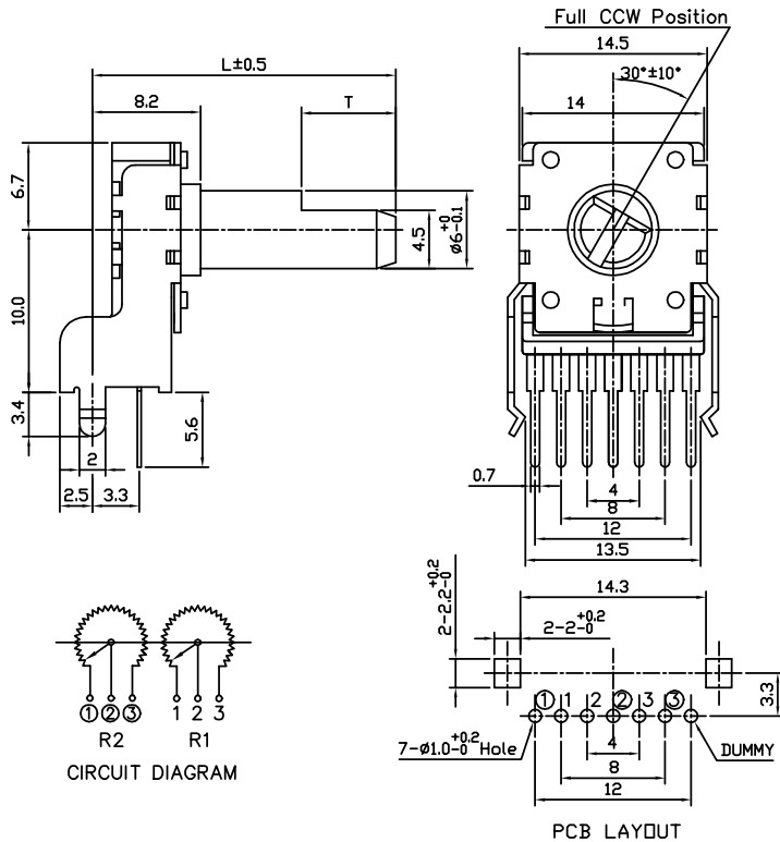
Model P140KV1 (Side Adjust, with Bushing)
