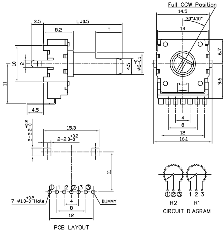
Model P140KH (Top Adjust, without Bushing)
