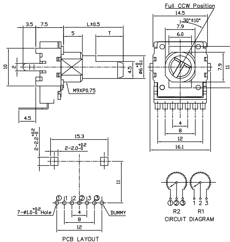
Model P140KH1 (Top Adjust, with Bushing)
